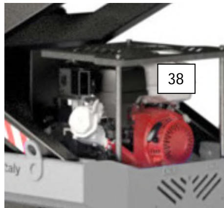
38. Brandstoftank
