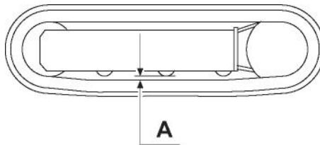
Fig. 174 Controle spanning rupsband 1
